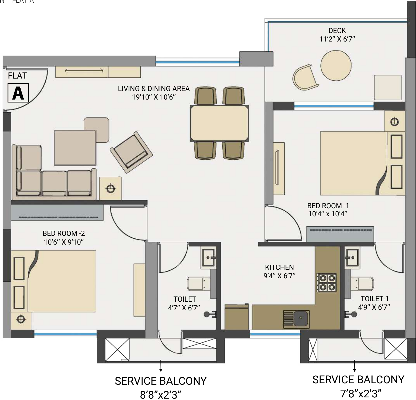
SMALL-TYPE APARTMENT UNIT PLAN – FLAT A
