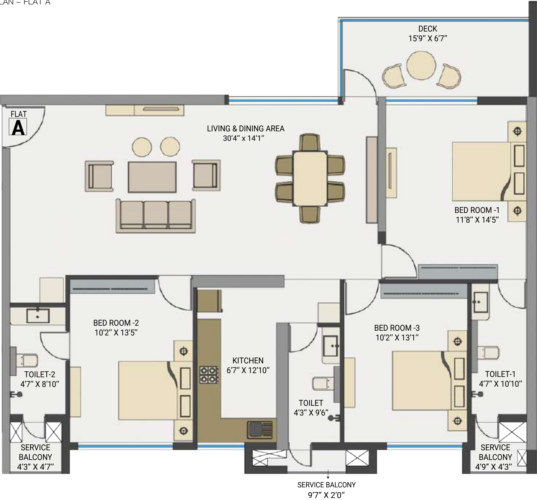
BIG-TYPE APARTMENT UNIT PLAN – FLAT A
