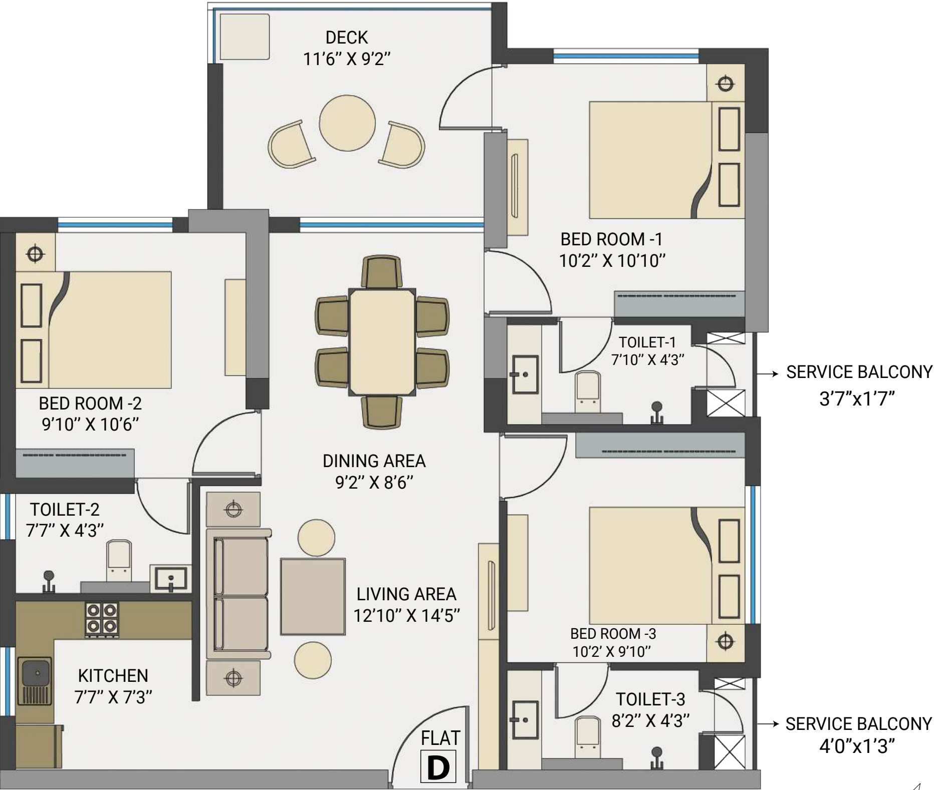
SMALL-TYPE APARTMENT UNIT PLAN – FLAT D
